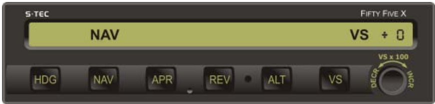
Fig. 2-11. AP Display, NAV and VS Modes Engaged, 0 FPM (Pre-Flight)
